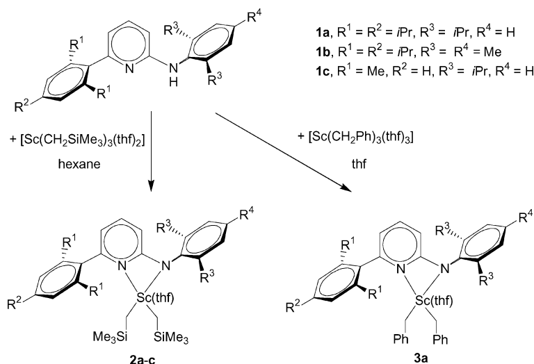
Scheme 1. Synthesis of Ap-stabilized dialkyl compounds 2a , 2b , 2c and 3a .
