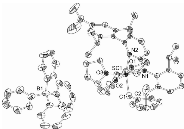
Figure 2. ORTEP diagram of the molecular structure of 4a in the solid state (ellipsoids set at 50% probability level). H Atoms have been omitted for clarity. Selected bond lengths [Å] and angles [°]: Sc1–C1 2.234(6), Sc1–N1 2.188(4), Sc1–N2 2.358(4), Sc1–O1 2.177(3), Sc1–O2 2.192(3), Sc1–O3 2.217(3), Sc1–C1–C2 121.2(4), O1–Sc1–C1 95.15(17), O2–Sc1–C1 89.51(17), O3–Sc1–C1 95.94(18).
