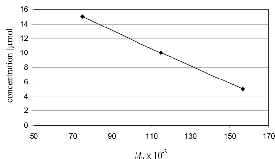
Figure 6. Plot of concentration of 2a vs. average number molecular weight ( M_n ) of the obtained polyisoprene.
