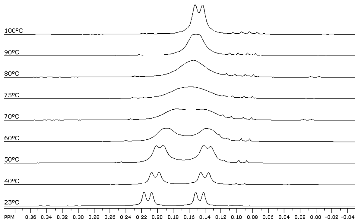
Figure 4. ^1\text{H} NMR spectra of 6a in [\text{D}_8]\text{toluene} at different temperatures.
