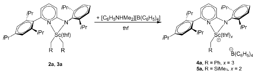
Scheme 2. Synthesis of organoscandium cations 4a and 5a .
