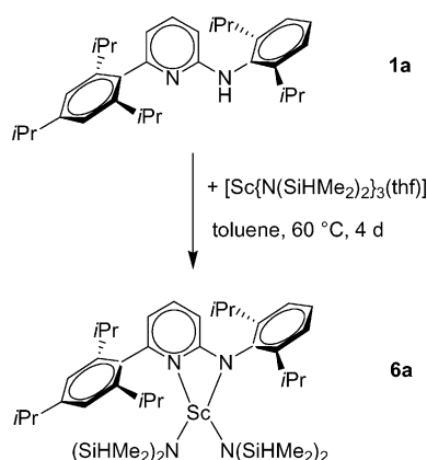
Scheme 3. Synthesis of the aminopyridinato-stabilized diamide 6a .
