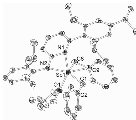
Figure 1. ORTEP diagram of the molecular structure of 3a in the solid state (ellipsoids set at 50% probability level). H atoms and solvent molecules have been omitted for clarity. Selected bond lengths [Å] and angles ^\circ : \text{Sc1}-\text{N1} 2.286(2) , \text{Sc1}-\text{N2} 2.1290(19) , \text{Sc1}-\text{C1} 2.245(3) , \text{Sc1}-\text{C8} 2.256(3) , \text{Sc1}-\text{C9} 2.657(2) , \text{N1}-\text{Sc1}-\text{N2} 61.31(7) , \text{Sc1}-\text{C1}-\text{C2} 121.88(16) , \text{Sc1}-\text{C8}-\text{C9} 88.50(15) .
