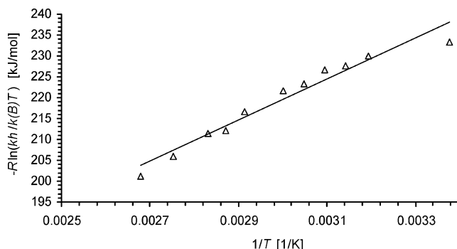
Figure 5. Eyring plot ( -R\ln(kh/k_B T) = -\Delta S^\ddagger + \Delta H^\ddagger/T ) for the coalescence of the SiMe signals.
