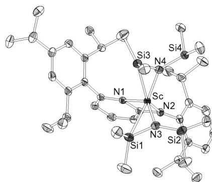
Figure 3. ORTEP diagram of the molecular structure of 6a in the solid state (ellipsoids set at 50% probability level). H Atoms have been omitted for clarity. Selected bond lengths [Å] and angles [°]: Sc–N1 2.2548(14), Sc–N2 2.1320(14), Sc–N3 2.0573(15), Sc–N4 2.0409(14), Sc–Si1 2.9003(6), Sc–Si2 3.4117(6), Sc–Si3 2.8642(6), Sc–Si4 3.4208(6), Si1–N3–Si2 129.45(9), Sc–N3–Si1 100.93(7), Sc–N3–Si2 129.36(9), Si3–N4–Si4 128.64(9), Sc–N4–Si3 99.40(7), Sc–N4–Si4 131.32(8), N1–Sc–N4 116.33(5), N3–Sc–N4 107.36(6), N2–Sc–N3 109.49(6).
